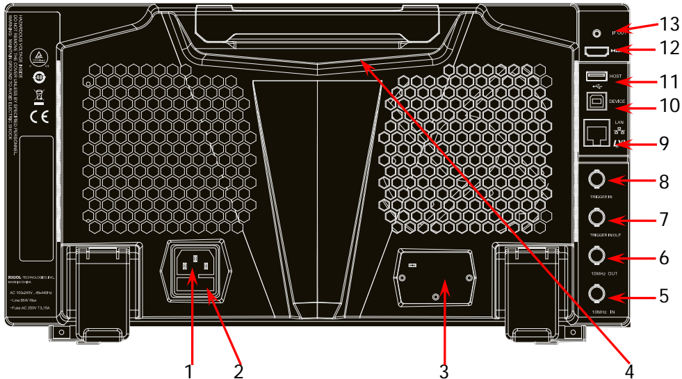
Figure 1-8 Rear Panel
