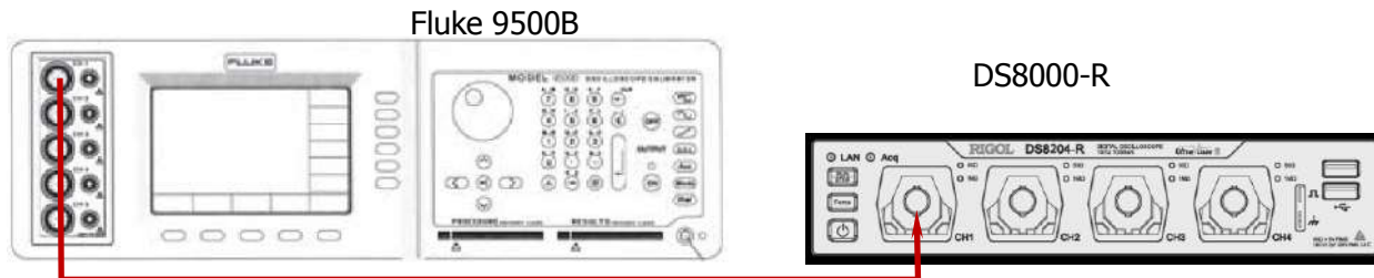
Figure 2-2 DC Gain Accuracy Test Connection Diagram
