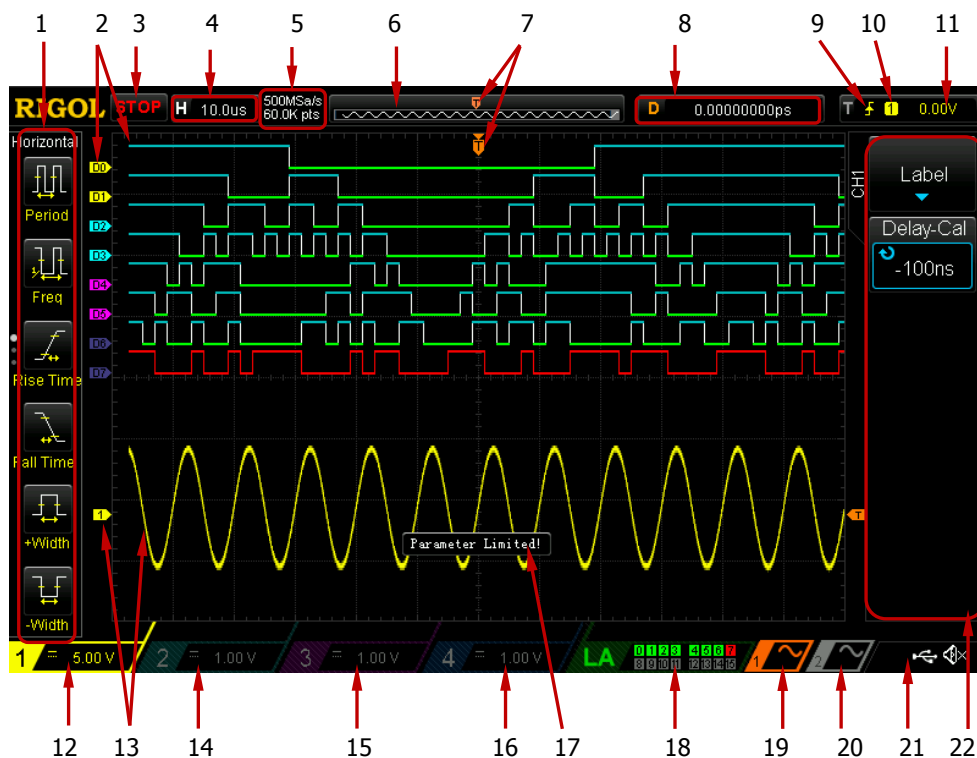
Figure 12 User Interface
